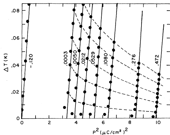
FIG. 2. Representative polarocaloric data showing the adiabatic temperature change from the initial temperature as a function of the square of the sample polarization. The solid lines show the extrapolations to a single domain at E=0 and are labeled by T_c - T at the initial point. The dashed lines show some isochoamps.
